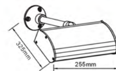
● SNLED-132B1 2 x 3W = 6W 6000K: 360Lm
