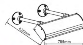
● SNLED-135B2 5 x 3W = 15W 6000K: 700Lm
