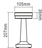
● ETLED-53E (Cade)
