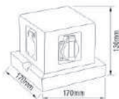
● YG-247-2 With 4 Sockets
