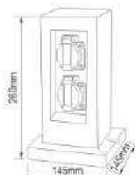
● YG-311-2 With 2 Sockets
